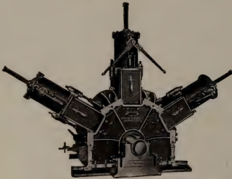
Patent Improved Wood Pulp Grinder.
